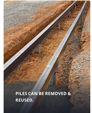
7" DIAMETER HELICAL PILING INSTALLED 30' FOR LAUNCHER/RECEIVER IN POOR SOILS
